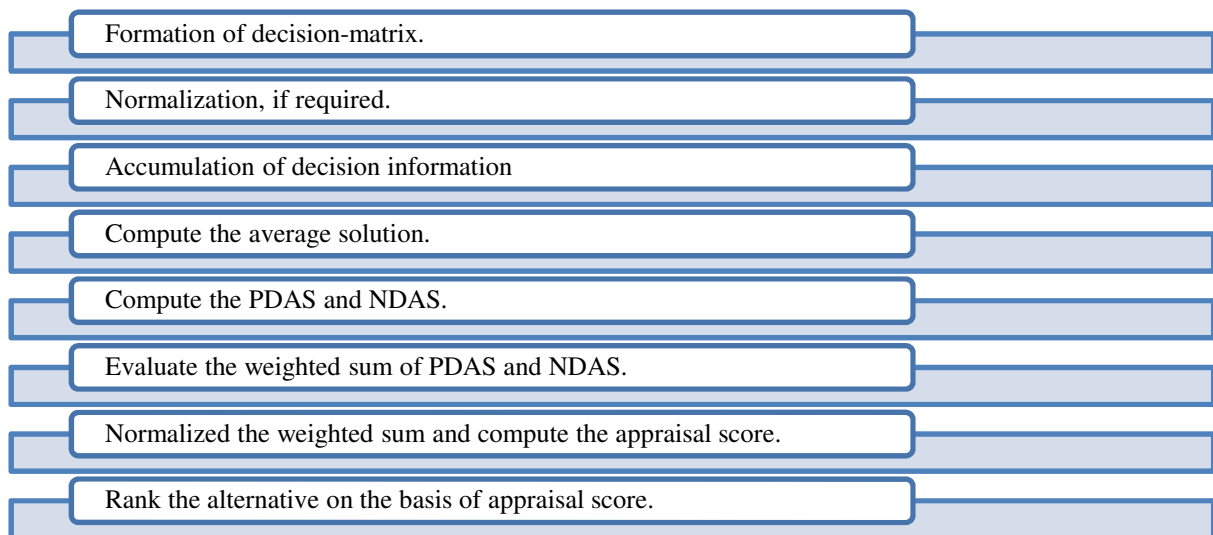
Fig. 1. Algorithm
