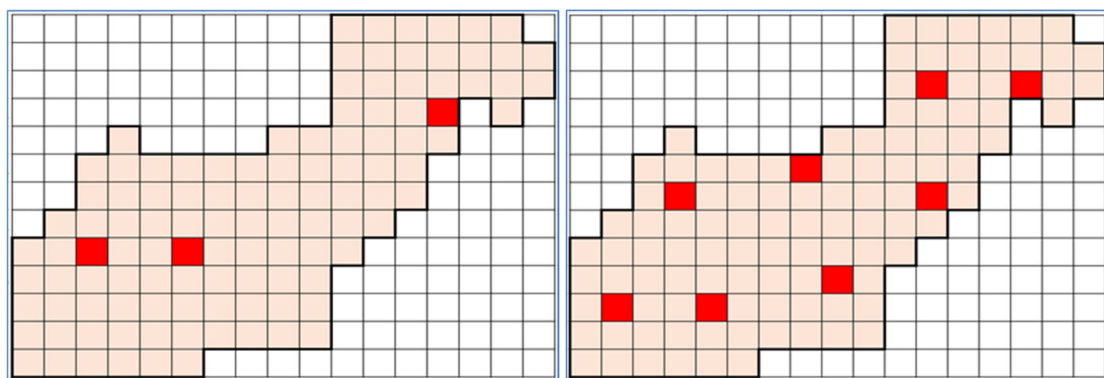
Fig. 5. Number of EMS required at 5 and 10 minutes response time
