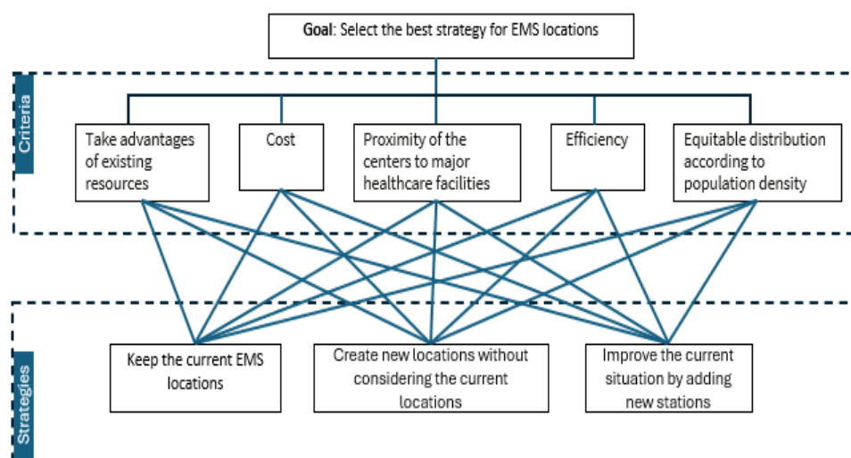
Fig. 9. Hierarchical structure of the case study
