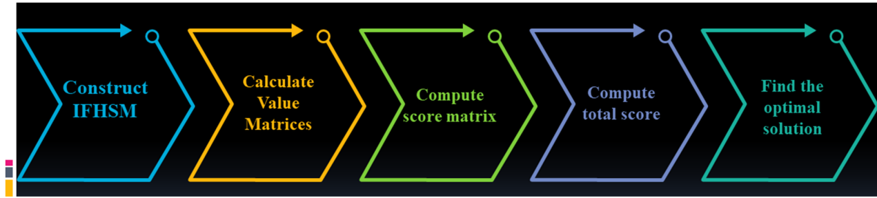
Fig. 1. Proposed algorithm
