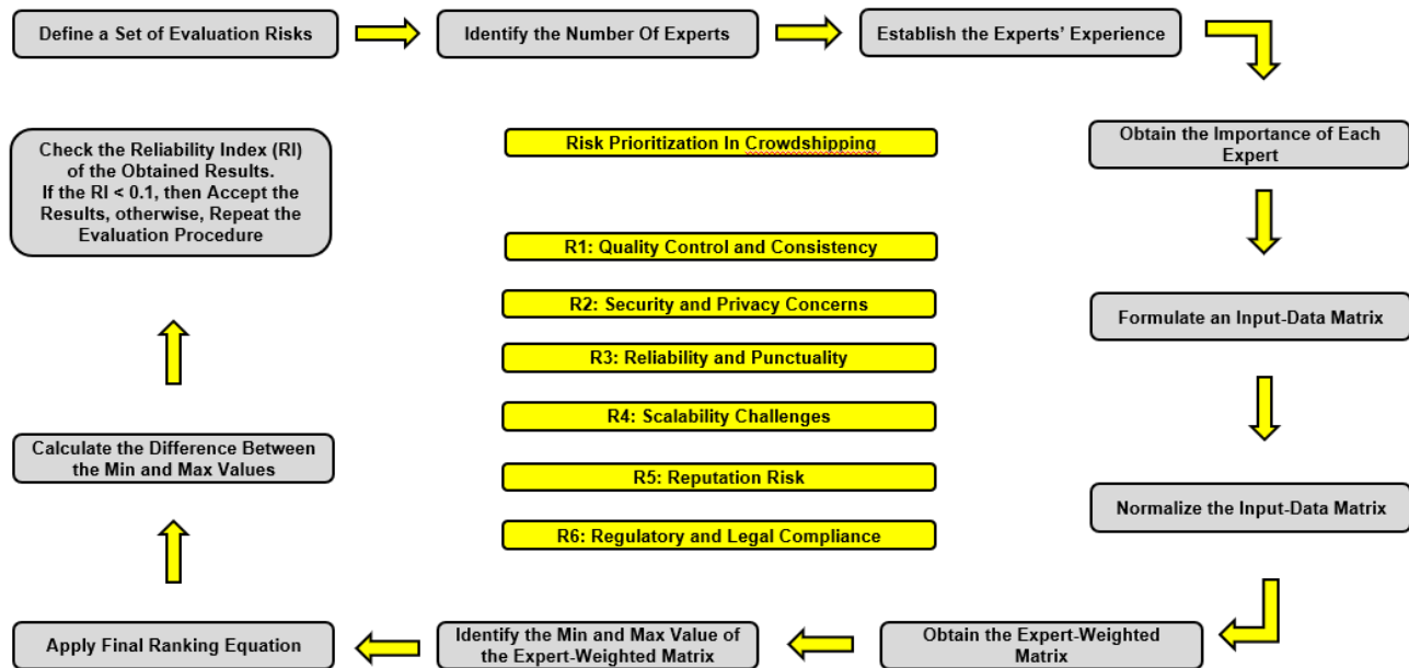
Fig. 1. Flowchart of the CIMAS methodology along with the established risks
